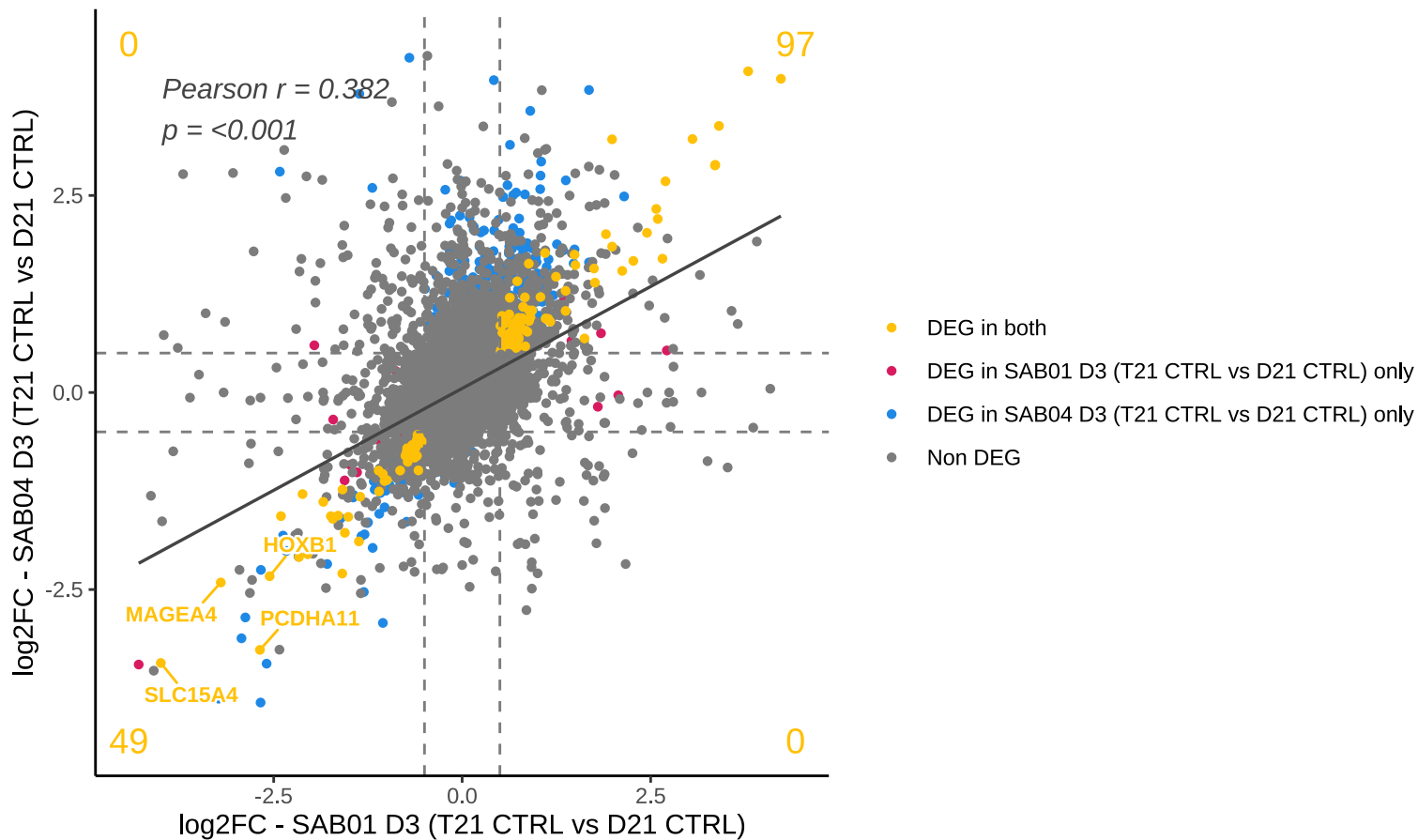
Comparison between SAB01 D3 (T21 CTRL vs D21 CTRL) and SAB04 D3 (T21 CTRL vs D21 CTRL)
